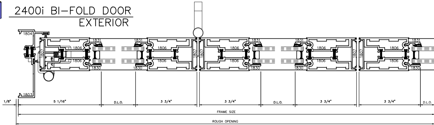
① HORIZONTAL SECTION
